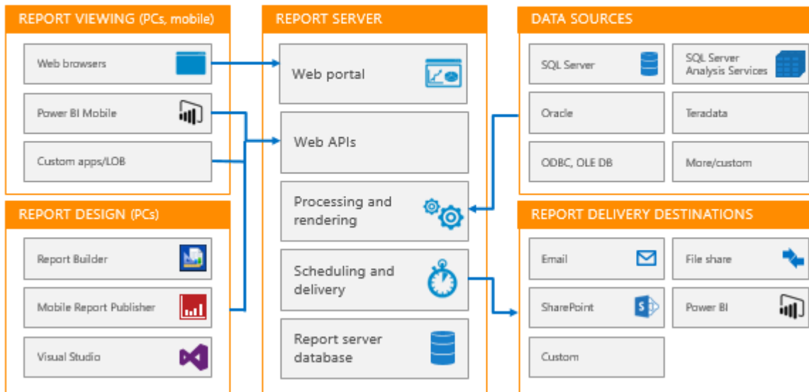
Figure 13: Reporting Services architecture
