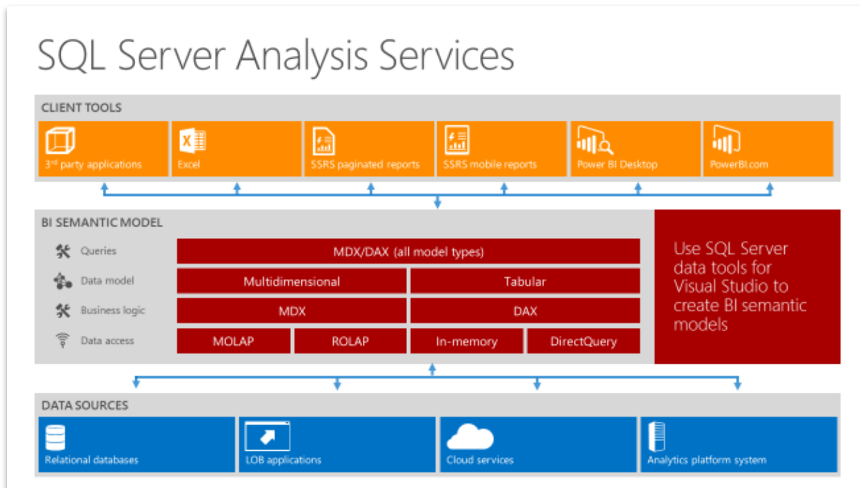
Figure 9: Capabilities of SQL Server Analysis Services
