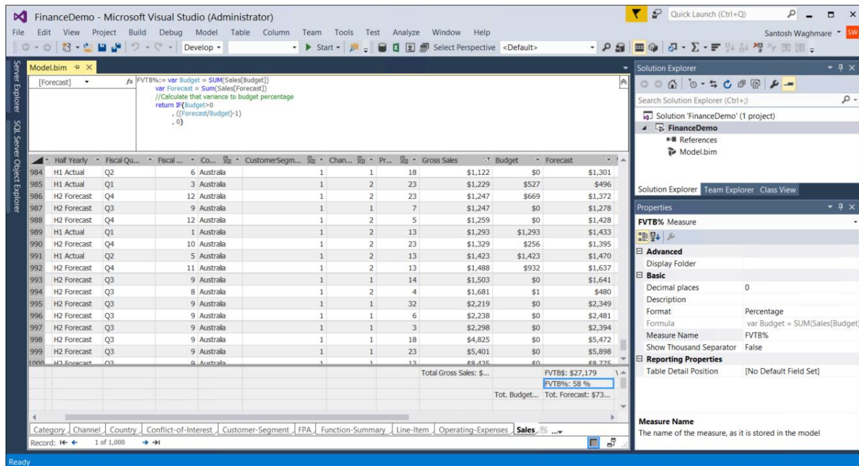
Figure 10: DAX support of named variables
