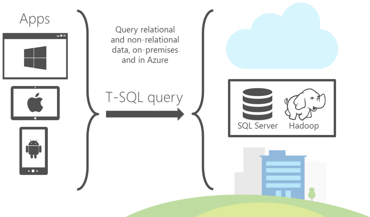
Figure 4: PolyBase access to distributed data sets
