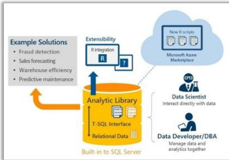
Figure 12: Near-database analytic scenarios
